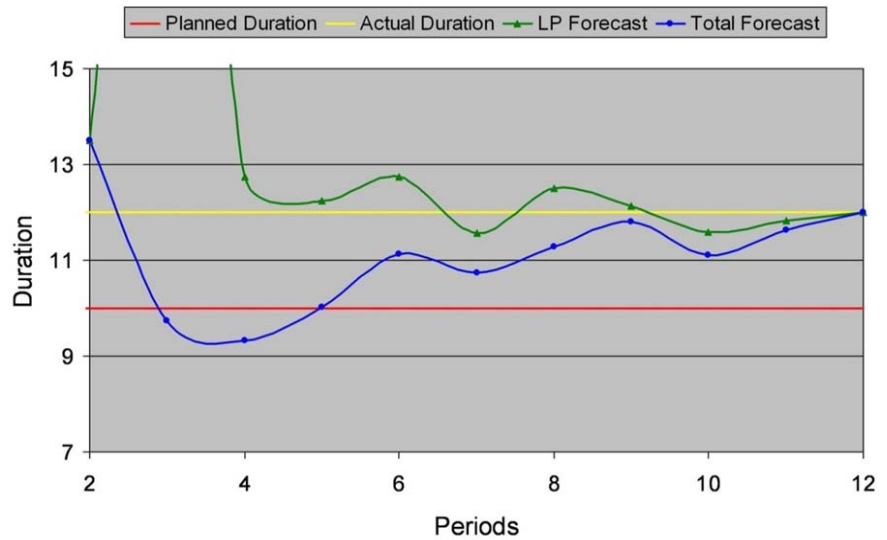
Figure 3. Longest Path Forecasting
