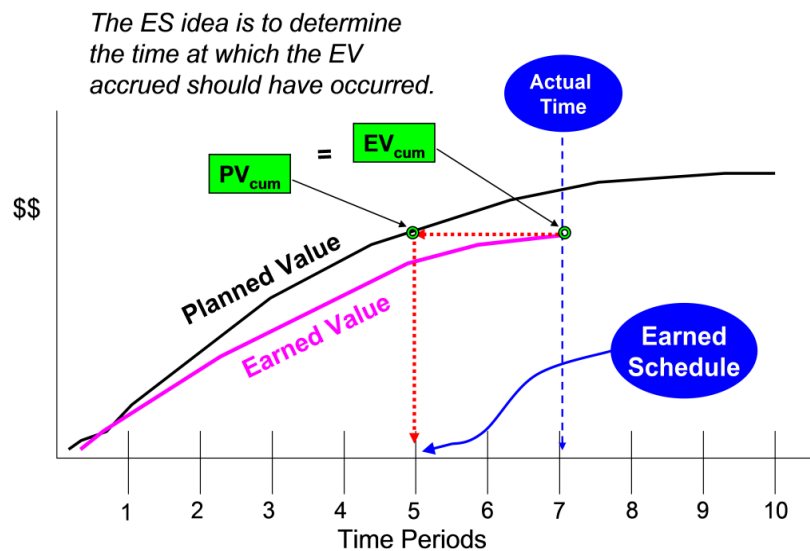
Figure 1. Earned Schedule Concept
