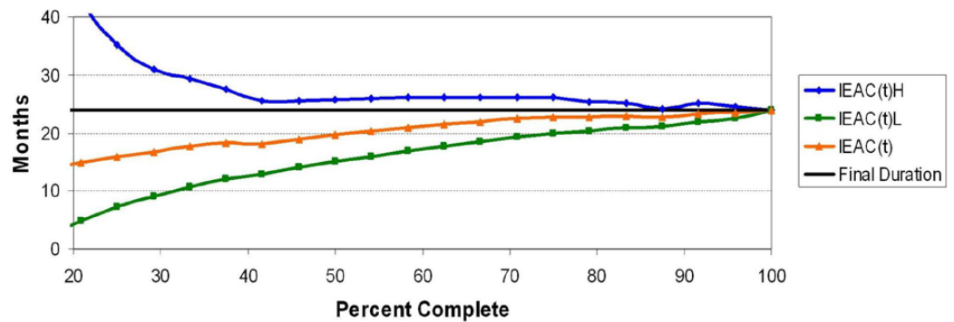
Figure 2. Statistical Forecasting
